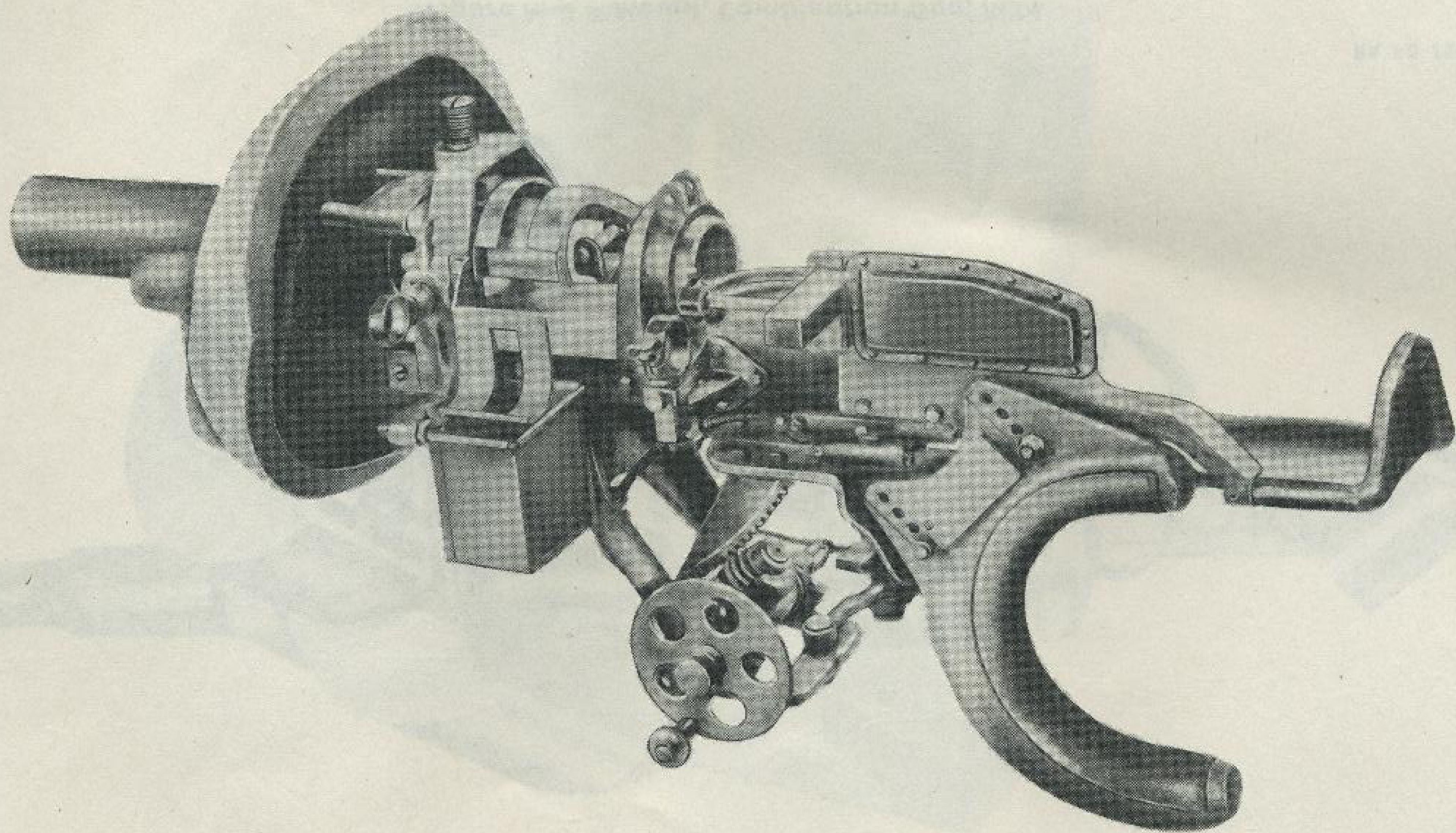
Figure M-3 — Mount, Combination Gun, M22
